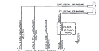
FIGURE 8 PEDAL CIRCUITS MODEL A CONSOLES SERIAL NO. 1 TO 2499 MODEL B AND BC CONSOLES SERIAL NO. 4000 TO 5075 (FOR PEDAL WIRING SEE FIGURE 13, COLUMNS 1,4,5,6,7,8,9)
