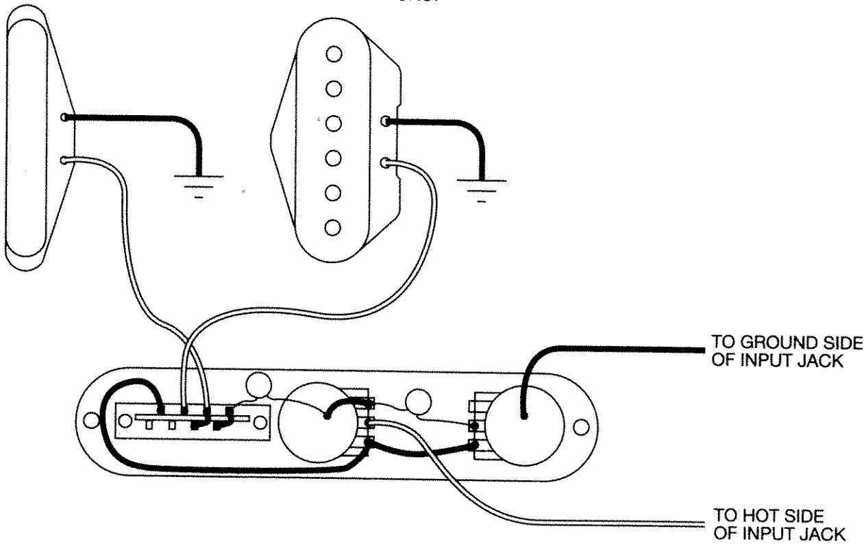
ORIGINAL VINTAGE TELE BRIDGE PICKUP
